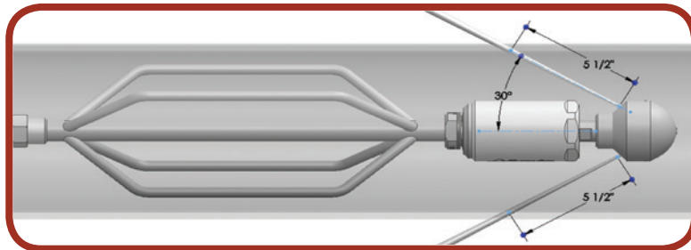
Figure 12-5b: With Centralizer- provides a uniform standoff distance
