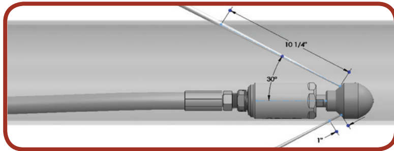
Figure 12-5a: Without Centralizer- results in a non-uniform standoff distance.
